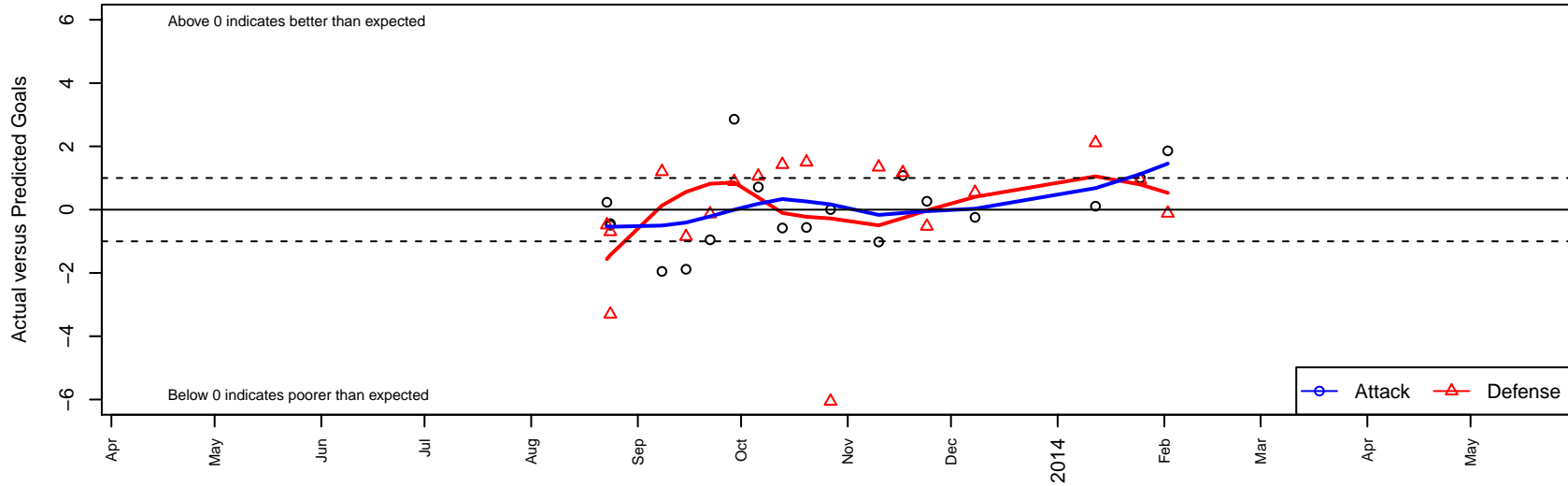
NWN Blue B95 Dots are actual minus expected GF (blue circles) and GA (red triangles). Blue line is smoothed change in attack strength. Red is smoothed change in defense strength.
